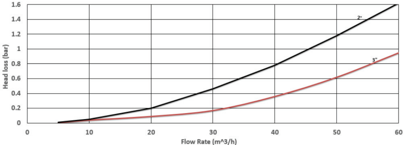
Adir TVD Automatic Disc Filter
